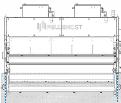
Conveyor version
