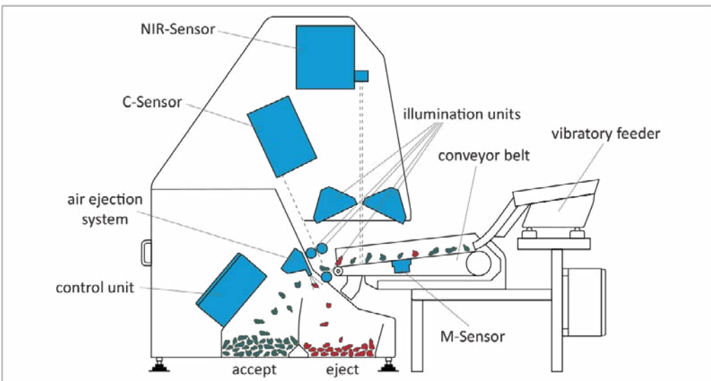
Function description: VARISORT COMPACT multi-sensor sorting machine
